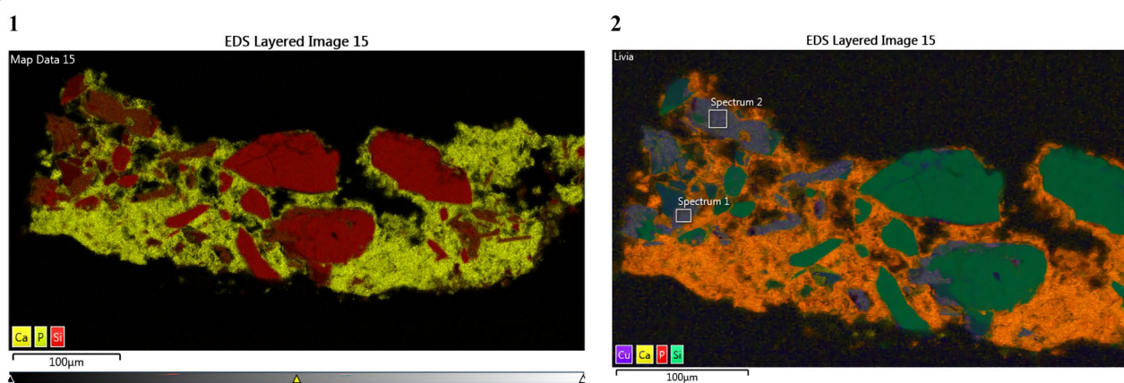
Fig. 6 1. Ca/P matrix and Si embedded grains. 2. Ca/P matrix and Si-Ca-Cu embedded grains with indication of EDS area analysis
