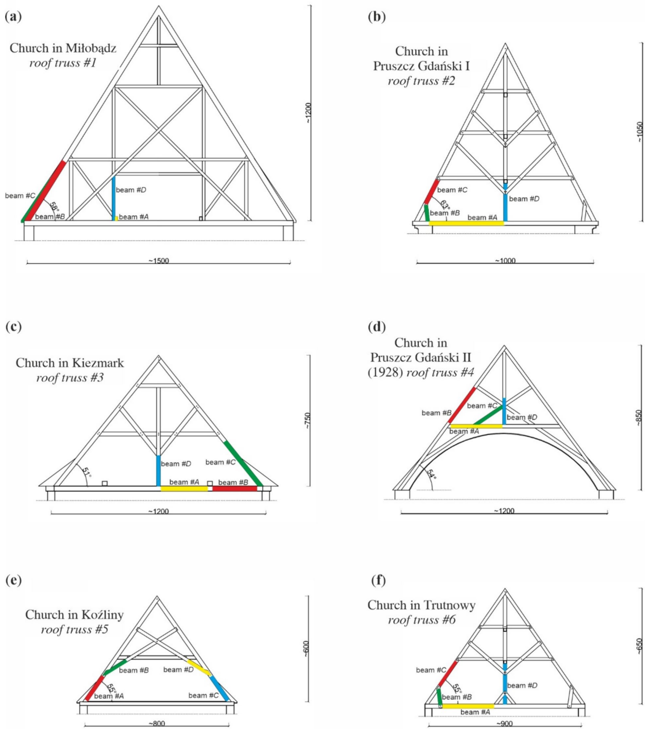
Fig. 4 Geometry and girders of the roof trusses with the indication of the measured timber elements, churches in: a Miłobądz (#1) b Pruszcz Gdański I (#2) c Kiezmark (#3) d Pruszcz Gdański II (#4) e Koźliny (#5) f Trutnowy (#6)
